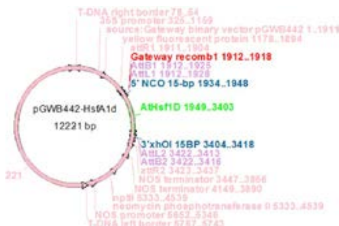
Figure 2: Diagrammatic representation of pGWB442-HsfA1d vector.
