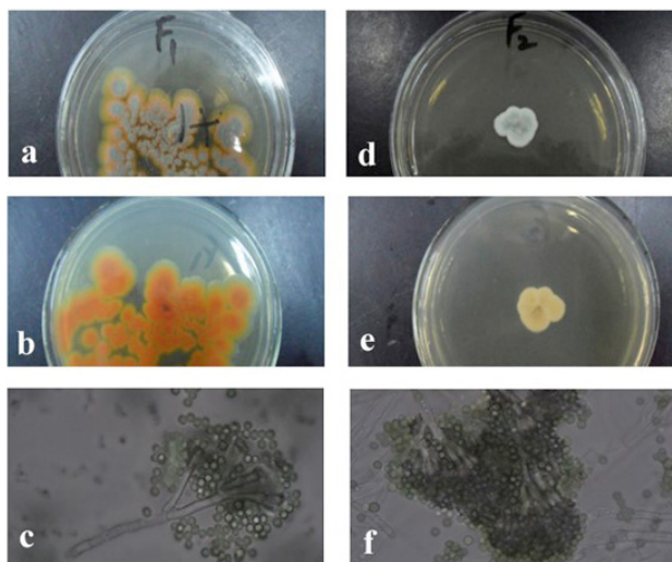
Fig. 1. The colony morphology of the strain F1 ( Penicillium viticola ) F2 ( Penicillium restrictum ) (a, front; b, back; c, mycelium and the chains of its conidia).
