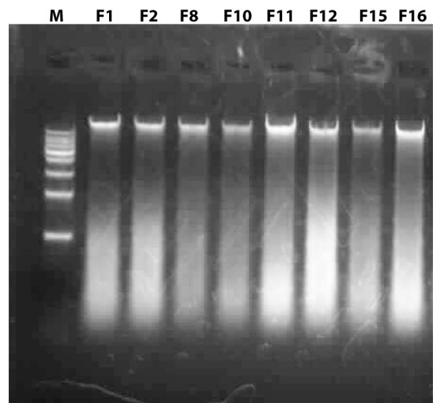
Fig. 5. Genomic DNAs of the fungal isolates; lane M: 1 kb DNA ladder, Lane F1, F2, F8, F10, F11, F12, F15, and F16 are the genomic DNAs of them.
