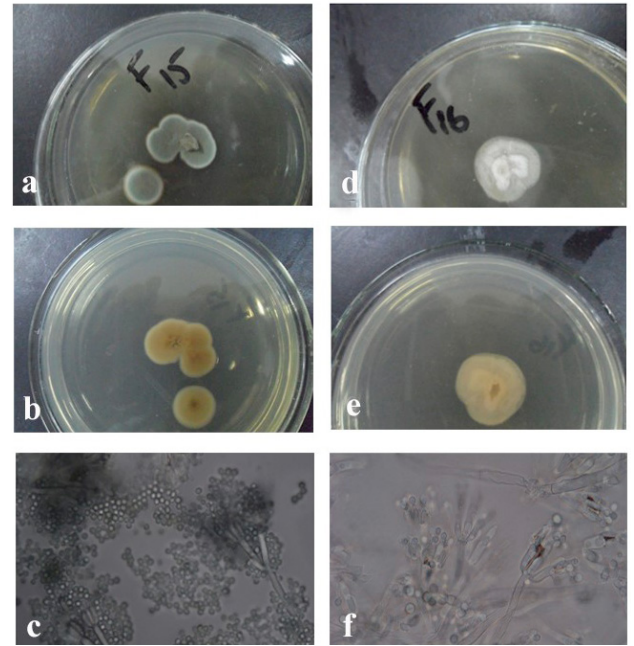
Fig. 4. The morphologies of the colony of the strain F15 ( Penicillium sumatrense ) (a, front; b, back; c, mycelium and the chains of its conidia); the strain F16 ( Penicillium vinaceum ) (d, front; e, back; f, mycelium and the chains of its conidia).
