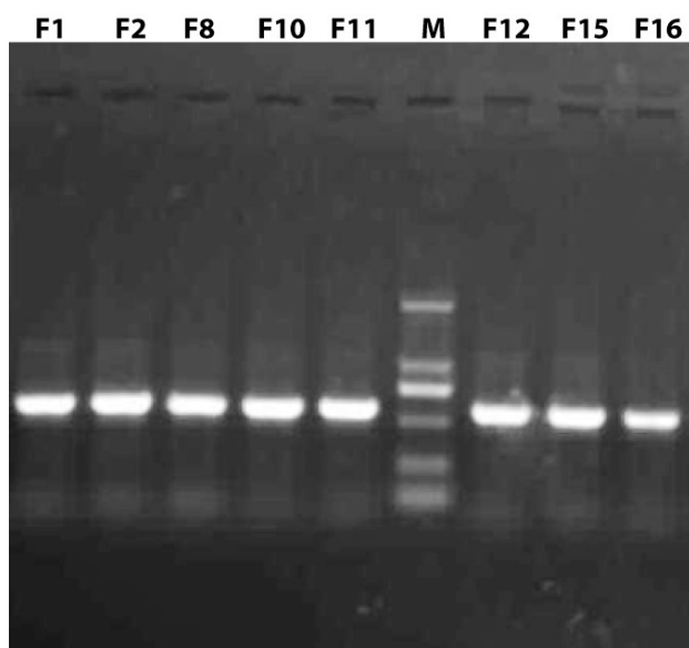
Fig. 6. Resolving pattern of PCR amplified ITS sequences on 1% Agarose gel; Lanes F1, F2, F8, F10, F11, F12, F15, and F16 showed PCR products of the fungal isolates and Line M: DNA ladder, fragment size from top to bottom is 2000bp, 1000bp, 750bp, 500bp, 250bp and 100bp.
