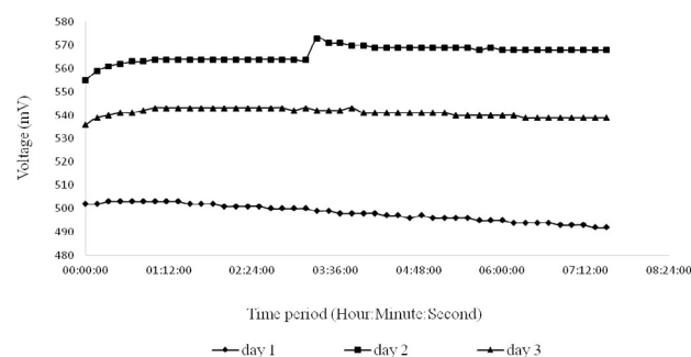
Fig. 3. Open circuit voltage of three days.
