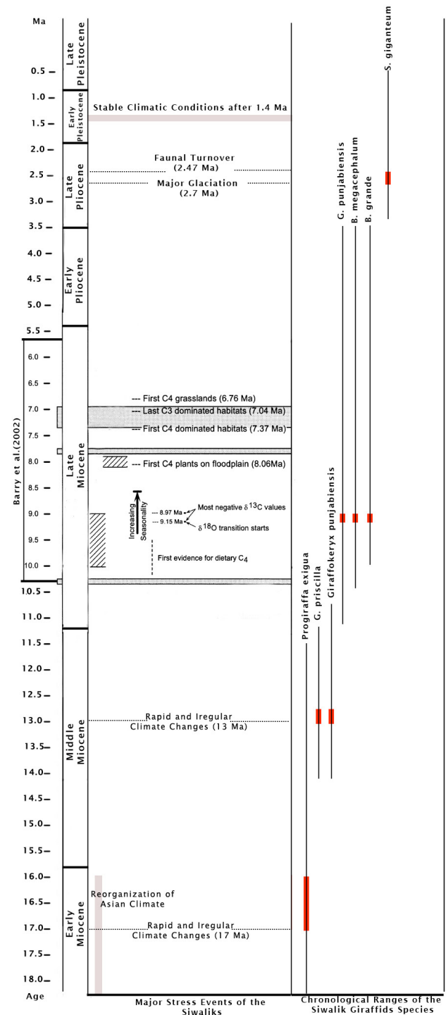
Fig. 5. Comparison of EH in giraffid species having different chronological distributions in the Siwaliks of Pakistan, Red areas in figure indicate the geological time for occurrence of EH in these species (Data for events and ages is taken from Barry and Flynn (1990), Barry et al. (2002), Dennell et al. (2006) and Lisiecki et al. (2007)).
