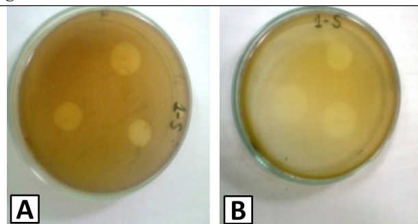
Figure 2: Zone of hydrolysis of BCTL- SL-197 after 24 h (A) and 48 h (B).
