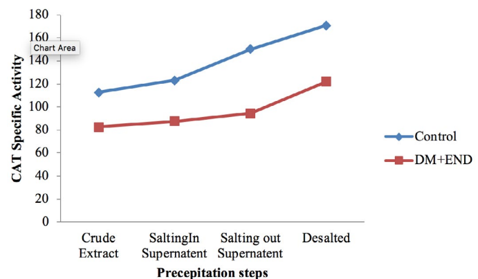
Figure 2: Partial purification of CAT specific activity from gills of Channa striata under insecticides mixture exposure.
