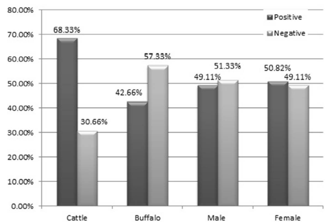
Fig. 1. Species and gender susceptibility of BEF in Punjab.
