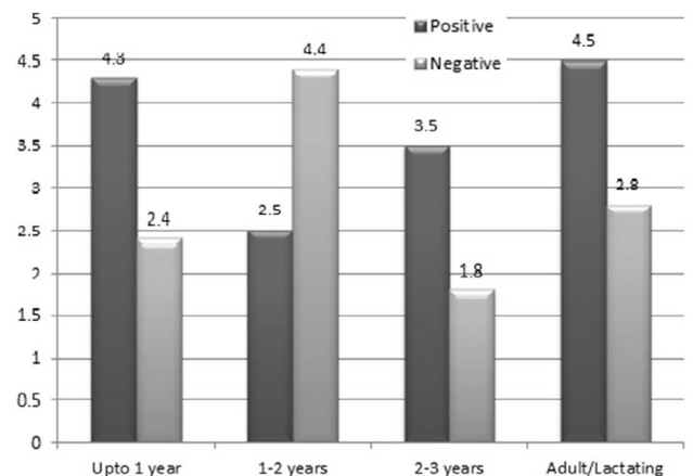
Fig. 2. Age susceptibility of BEF in bovines of Punjab.
