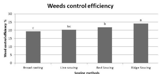
Figure 5: Weed control efficiency of different sowing methods of wheat.
