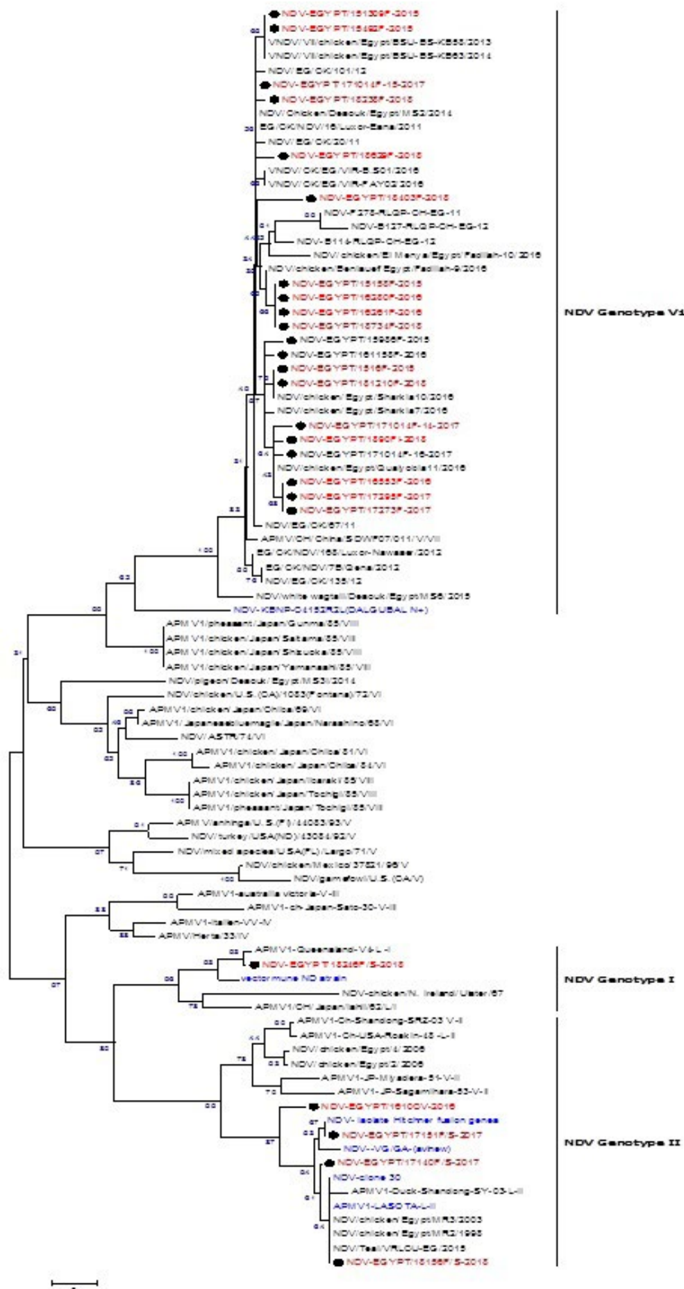
Figure 3: Phylogenetic tree of nucleotide sequences of the partial fusion gene fragment of Egyptian isolates (marked with a solid black circle) and the references strains from GenBank using neighbor-joining methods of Mega6 software.
