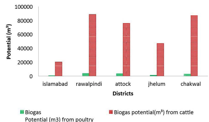
Figure 6: Biogas potential in different districts of Pothohar.
