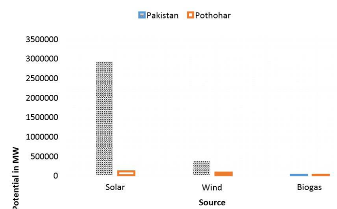
Figure 10: Total Solar and Wind energy potential in Pakistan and Pothohar.
