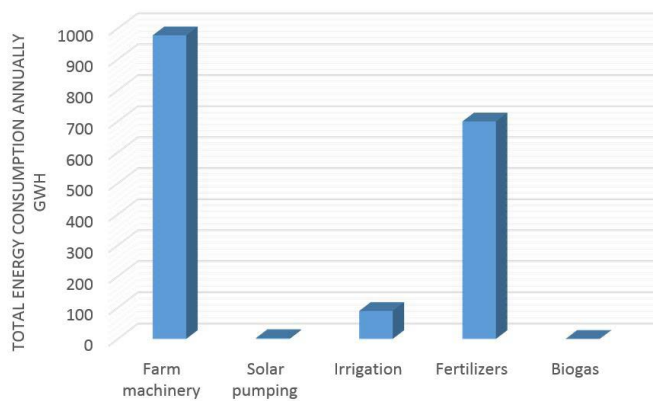
Figure 12: Total energy consumption annually (GWh).
