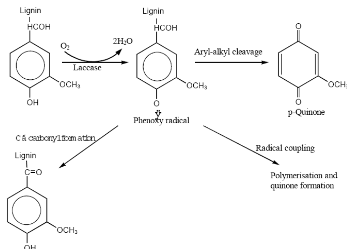
Figure 2: Laccase action on lignin, phenolic sub-units oxidation (adapted from Archibald et al. , 1997).
