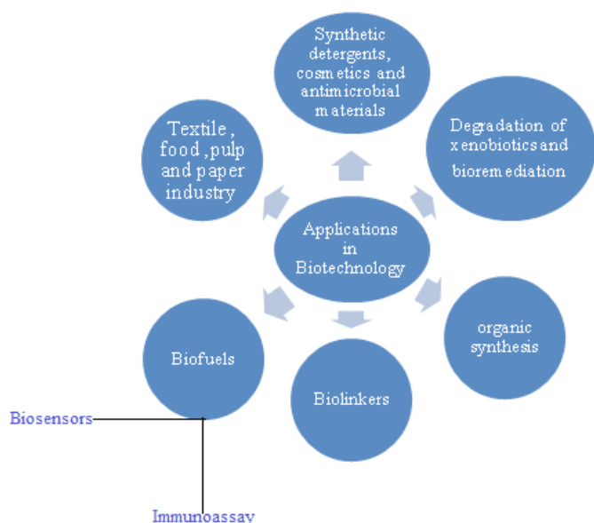
Figure 3: Scheme of applications of laccase (adapted from Morozova et al. , 2007).
