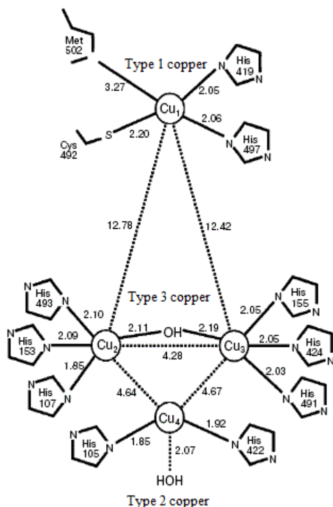
Figure 1: Scheme of T1 and T2/T3 copper sites of laccase (CotA) from Bacillus subtilis (modified from Enguita et al. , 2003).
