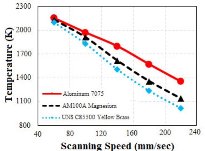
Figure 6: The temperature at the focus point of 1\mu\text{m} diameter grain.
