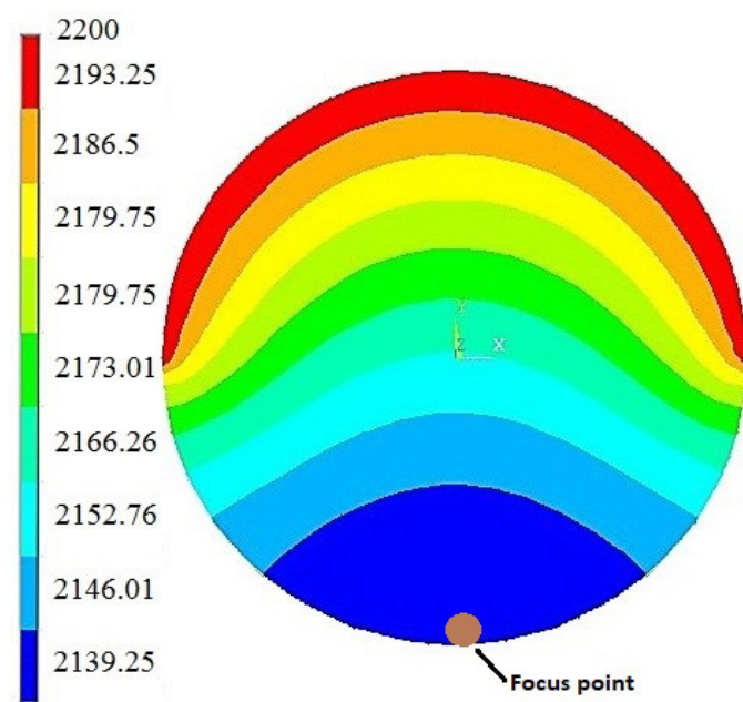
Figure 5: Temperature distribution on 1\mu\text{m} powder grain of Aluminum 7075 at 60 mm/sec scanning speed.
