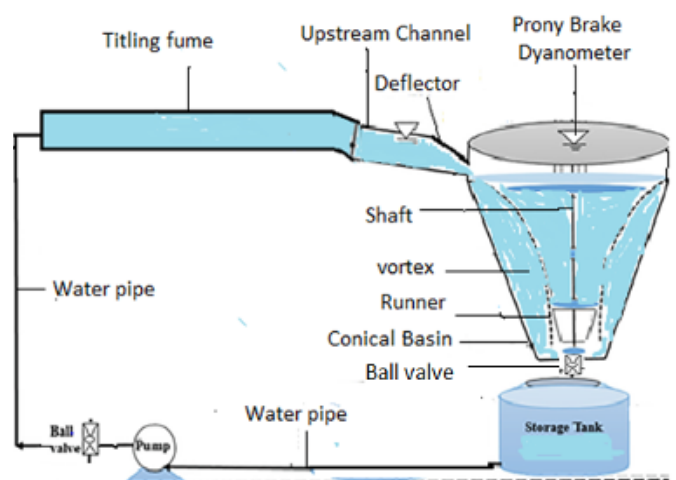
Figure 9: Schematic of GWVPP Set up.
