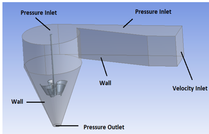
Figure 5: Boundary condition of GWVPP model.
