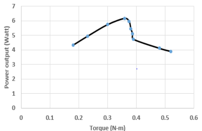
Figure 11: Torque vs power output (Watt).
