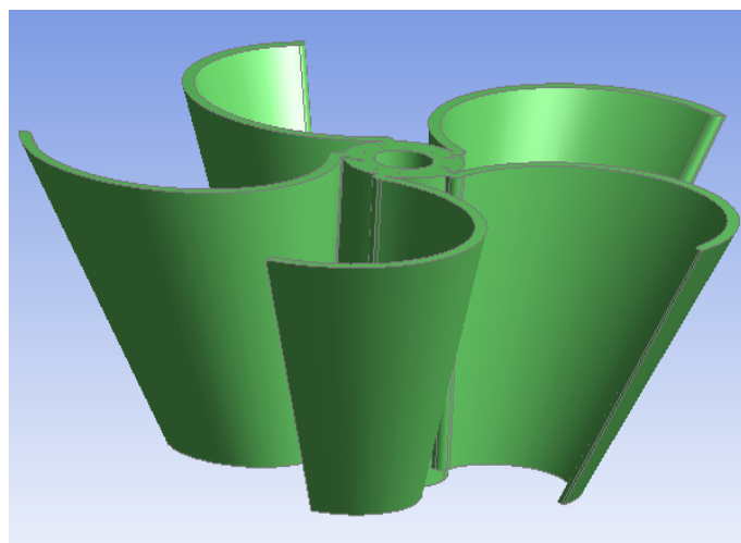
Figure 6: Proposed Novel runner of GWVPP.
