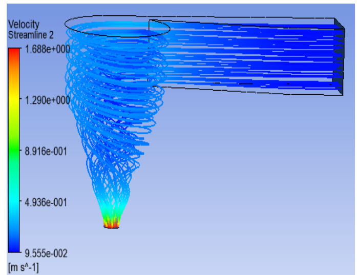
Figure 7: Velocity streamlines analysis of GWVPP Model with inside novel runner.
