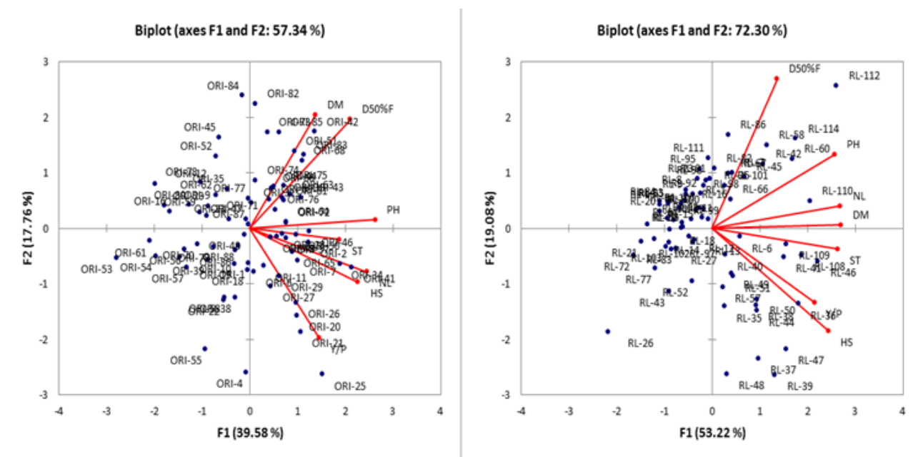
Figure 1: Biplot of different morphological traits for B-lines and R-lines of sunflower.
