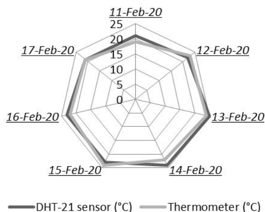
Figure 5: Temperature comparison for tunnel 1.
