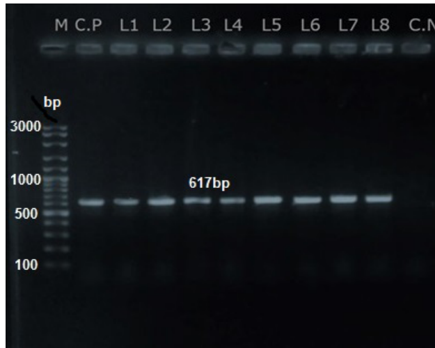
Fig. 1. Agarose gel electrophoresis of PCR products of stn gene. Lane M, molecular weight marker (100-3000bp); Lane C.P, control positive of S. Typhimurium reference strain (ATCC. 14028); Lanes 1-8, positive samples with band of amplicon size 617bp; Lane C.N, control negative (sterile nuclease free water).
