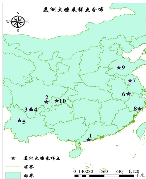
Fig. 1. Sampling sites: 1, Yangjiang county, Guangdong province (GDYJ); 2, Rong county, Zigong city, Sichuan province (ZGRX); 3, Xichang city, Liangshan prefecture, Sichuan province (LSXC); 4, Lizhou county, Liangshan prefecture, Sichuan province (LSLZ); 5, Dali city, Yunnan province (YNDL); 6, Xuancheng city, Anhui province (AHXC); 7, Huai'an city, Jiangsu province (JSHA); 8, Wenzhou city, Zhejiang province (ZJWZ); 9, Tai'an City, Shandong province (SDTA); 10, Chongqing Municipality (ZGCQ).
