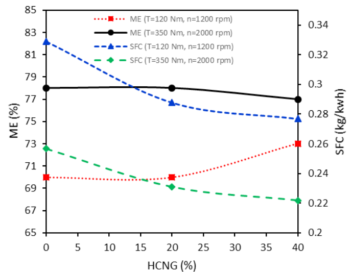
Figure 6: Effect of HCNG on ME and SFC.
