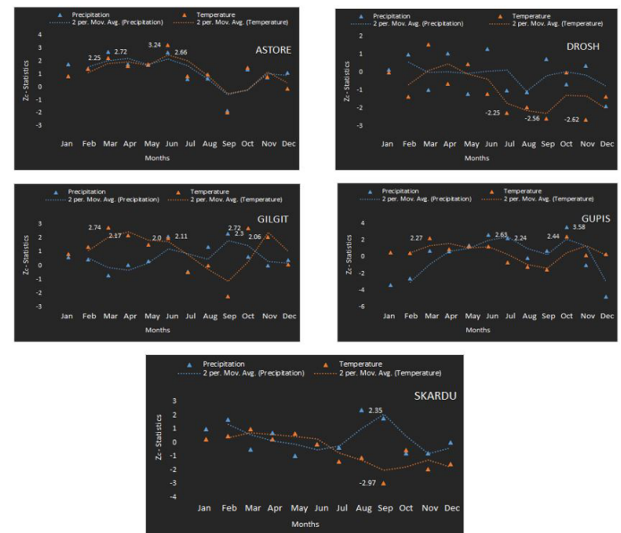
Figure 3: Overall moving average trend of the five selected sub-basins of UIB, Pakistan.
