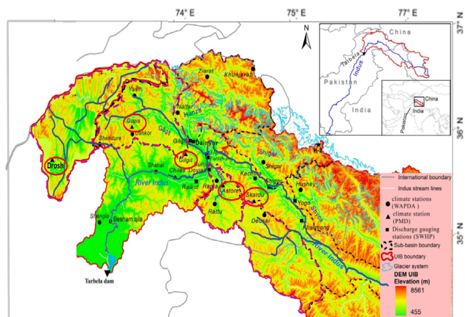
Figure 2: Climatic stations in Upper Indus Basin.
