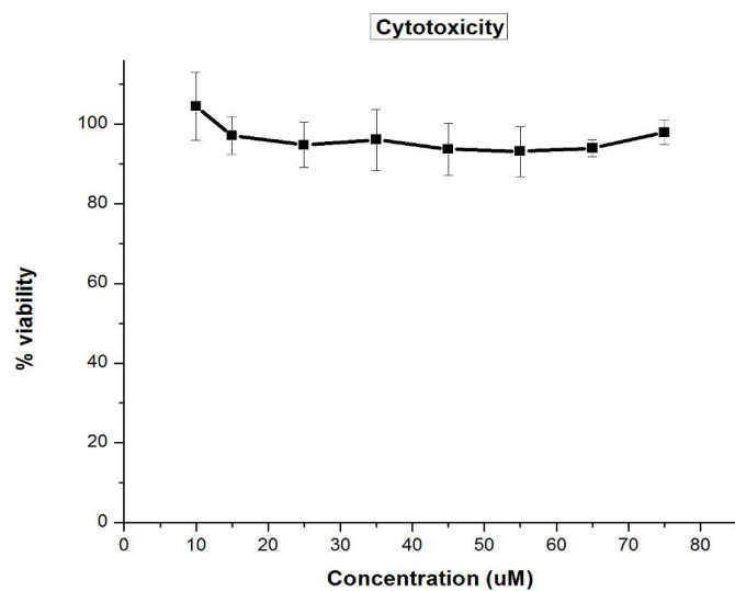
Figure 5: The cytotoxicity at different Photosense concentrations.
