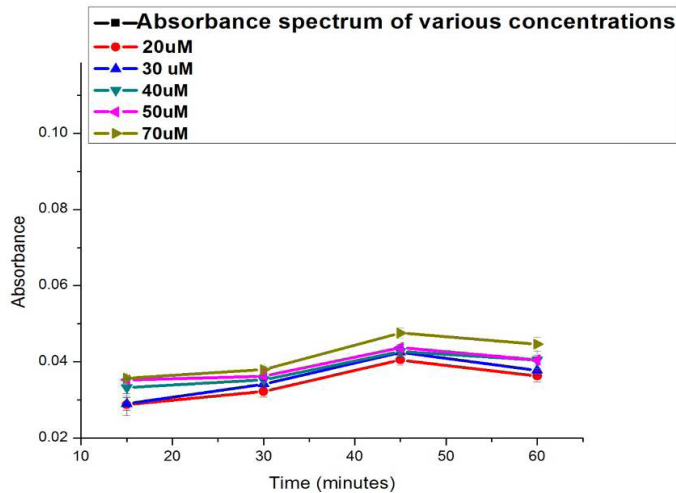
Figure 4: Absorbance spectrum of various concentrations.
