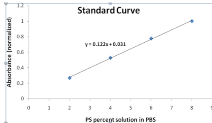
Figure 3: Standard curve of photosence.
