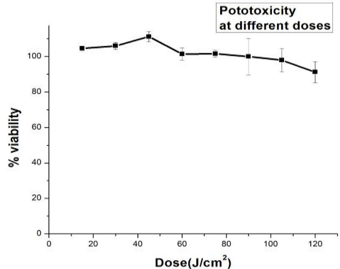
Figure 6: Phtotoxicity of different doses.
