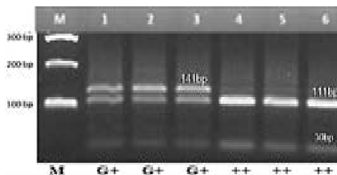
Figure 2: PCR-RFLP product of BMP15|HinfI gene (lines 1- 6) and marker 100 bp (M)
