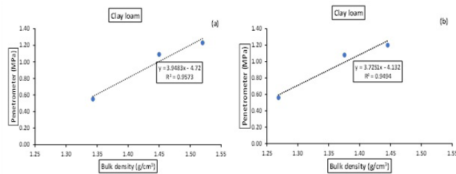
Figure 3: Relationship between dry bulk density under different compactions and soil penetration resistance for clay loam ( S_1 ) soil during (a) 2017-18 and (b) 2018-19 cropping seasons.
