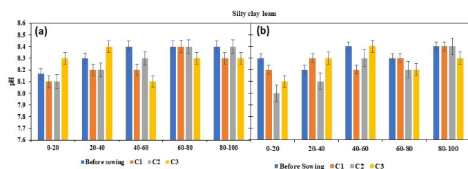
Figure 10: Before sowing and after experiment pH of silty clay loam ( S_2 ) soil under different compaction during 2017-18 (a) and 2018-19 (b) cropping seasons.
