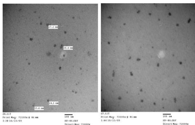
Figure 2: TEM image of spherical Nano-MO with an average size 24.1 nm
