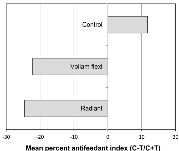
Figure 1: Antifeedant activity of two insecticides against Spodoptera frugiperda , showing the percent of feeding deterrence after 48 h. C, control; T, treated.
