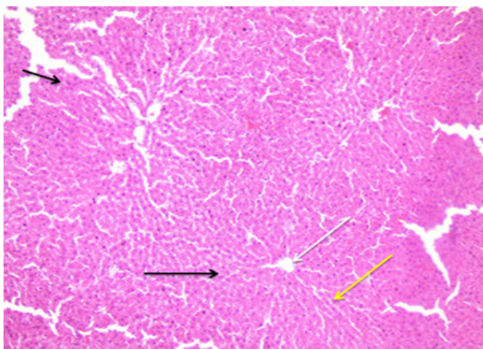
Figure 1: Photomicrograph of rats liver tissue section from Aloe group, showed hepatic tissue with normal liver lobules (black arrow), normal hepatocytes arrangements radiating (yellow arrow), around central vein (white arrow) (H and E, 10X).
