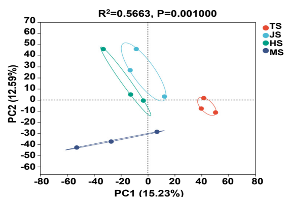
Fig. 1. Principal component analysis (PCA) based on Bray-Curtis Distance Matrix for soil samples collected from the rhizosphere of the four different stages.
