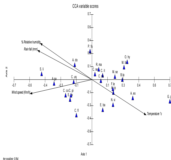
Figure 4: Canonical corresponding analysis (CCA), ordination biplot showing the association of abundant species towards Fodder crop.
