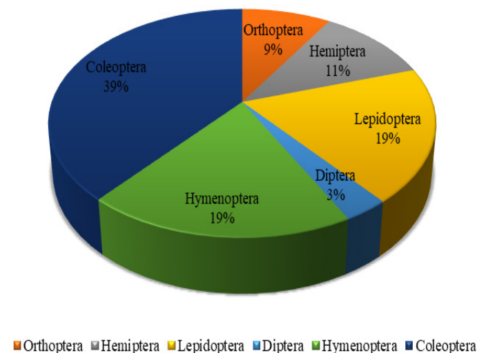
Figure 1: Order wise abundance of insects from Trifolium alexandrinum .
