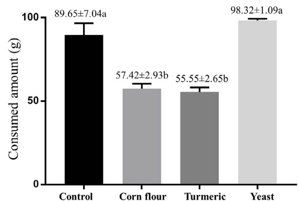
Fig. 2. The amount of each feeding type consumed after 72h (mean \pm SE). Letters denote the significant differences between feeding types according to Tukey test.
