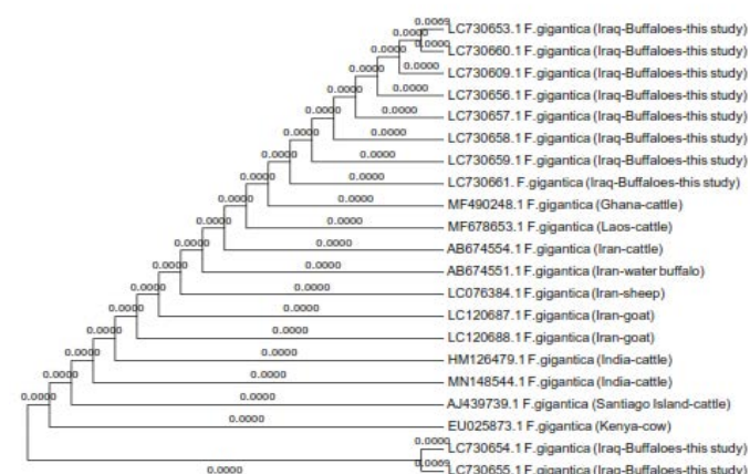
Figure 4: Comparison of phylogenetic analysis of 28S rRNA gene sequences of F. gigantica isolated from buffaloes liver from Iraq (present study) with other sequences recorded in Genbank.
