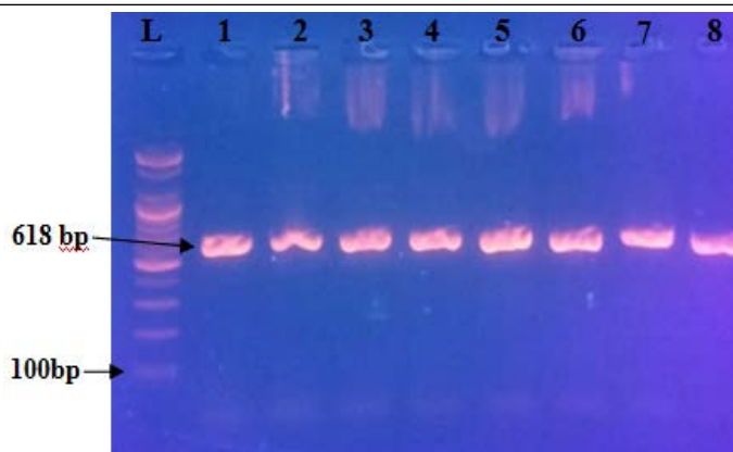
Figure 2: Electrophoresis of 28S rRNA gene. L: DNA Ladder. Lane 1-4 F. gigantica isolated from cows. Lane 5-8 F. gigantica isolated from buffaloes.
