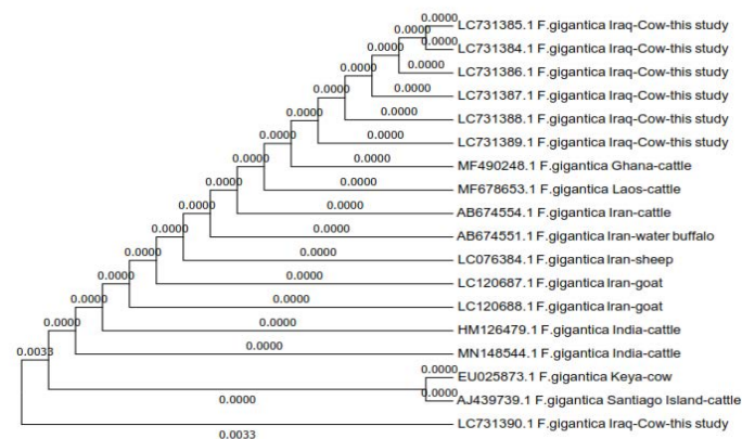
Figure 3: Comparison of phylogenetic analysis of 28S rRNA gene sequences of F. gigantica isolated from cows liver from Iraq (present study) with other sequences recorded in Genbank.
