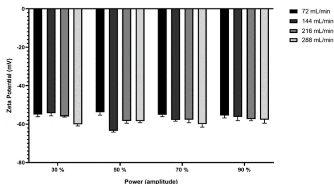
Figure 3: The zeta potential of a flow cell sonicator's BSO alginate nanoemulsion at various flow rates and power (amplitude). Data are shown as mean \pm SD (error bar) ( n=3 ).
