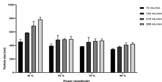
Figure 1: The BSO alginate nanoemulsion particle size of a flow cell sonicator at various flow rates and power (amplitude). Data are shown as mean ± SD (error bar) (n=3).
