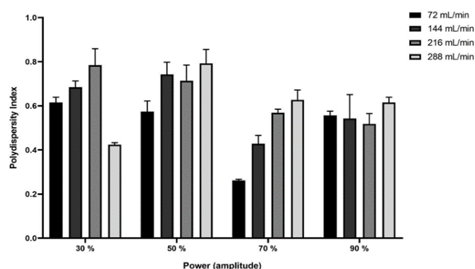
Figure 2: The flow cell sonicator's PdI of BSO alginate nanoemulsion at various flow rates and power (amplitude). Data are shown as mean \pm SD (error bar) ( n=3 ).
