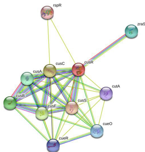
Fig. 5. CusR protein-protein interaction analysis through STRING server shows its major role in copper homeostasis (via Cus, Cue and Cut factors) in addition to regulation and sensing of some other heavy metals (via zraS ) as well as starvation (via rspR ).
