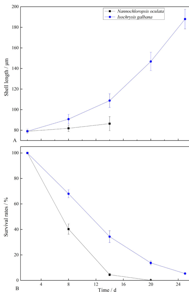
Fig. 4. The effects of growth and survival rates of larvae when fed N. oculata and I. galbana , respectively. (A) The effect of growth when fed N. oculata and I. galbana , respectively; (B) The effect of survival rates when fed N. oculata and I. galbana , respectively.
