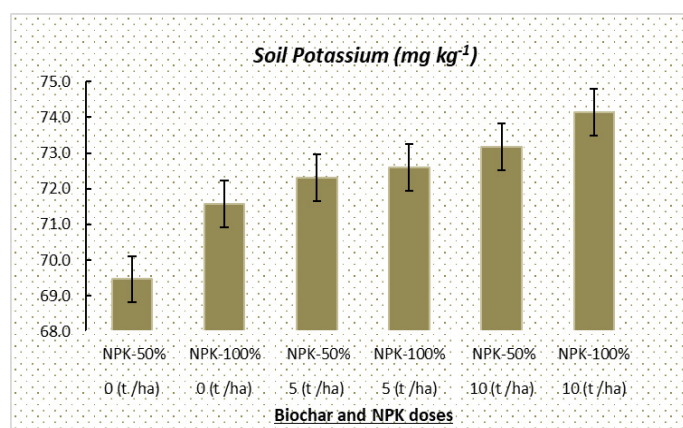
Figure 7: Graphical representation of Extr. soil potassium ( \text{mg kg}^{-1} ), influenced by biochar and NPK fertilizers under maize crop.
