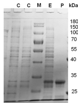
Fig. 1. SDS-PAGE showing the expression and purification of \alpha -glucosidase. Lane C, a control experiment (without the gene), Lane-M, Protein marker (ThermoFisher - unstained protein ruler). Lane E, experimental with the expression of the gene. P, purified enzyme, the molecular weight of the purified enzyme was found as 30 kDa.
