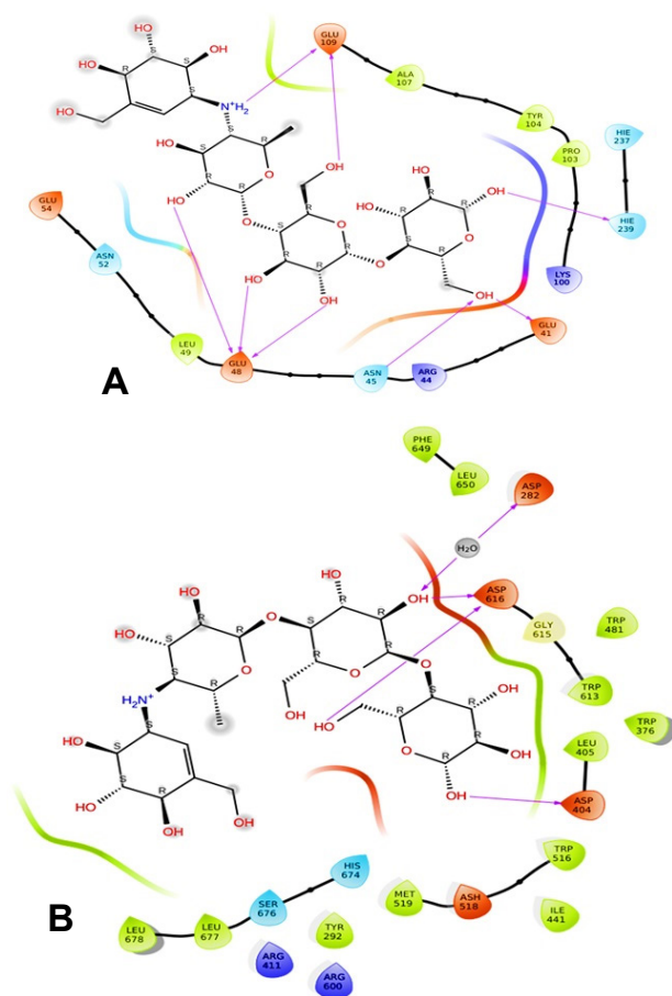
Fig. 4. Depicts a 2D interaction of \alpha -glucosidase and acarbose. A, enlarged model of the complex, highlighting the ligand in the active site of bacterial \alpha -glucosidase. B, provides a closer view of the complex, with the ligand displayed in the center of human \alpha -glucosidase.
