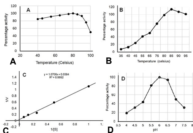
Fig. 2. A study of the kinetics of recombinant \alpha -glucosidase. A, Enzyme stability against temperature. B, Effects of temperature on enzyme activity. C, Lineweaver-Burk plot for K_m and V_{max} . D, Effects of pH on enzyme activity.
