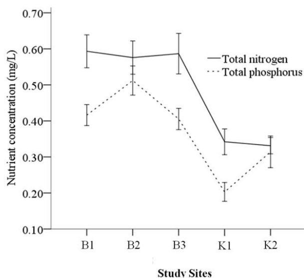
Fig. 4. Mean concentrations of total nitrogen and total phosphorus in five studied sites of East Kolkata Wetlands, India. Error bars represent standard error.
