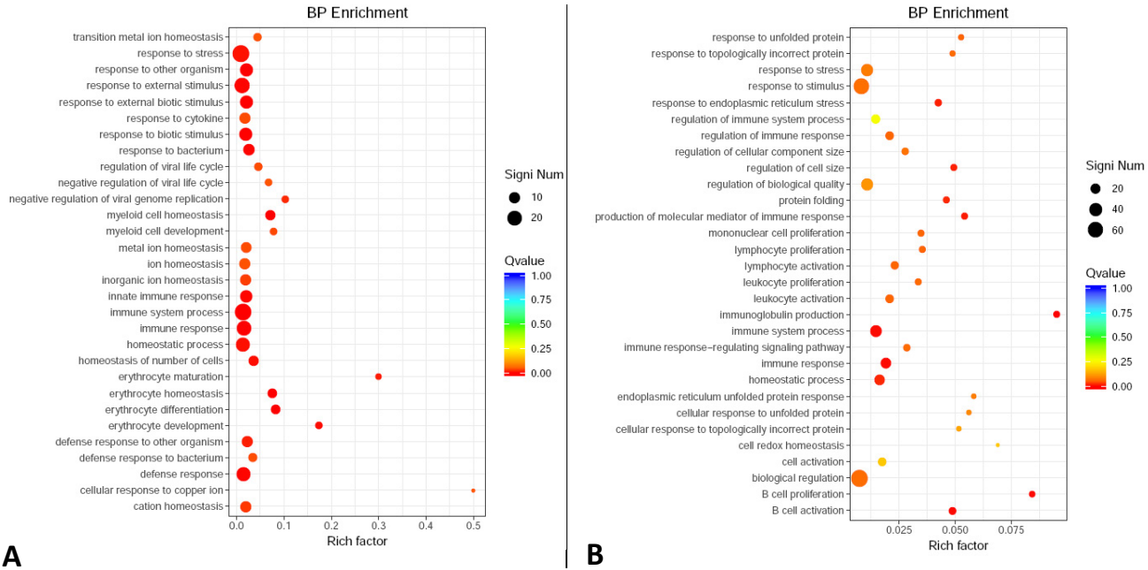
Fig. 3. Enriched functions in BP category of GO annotation for up-regulated (A) and down-regulated (B) DEGs of old SCTs as compared with cubs. For details of X-axis, Y-axis, Q value and DEGs, see Fig. 2.
