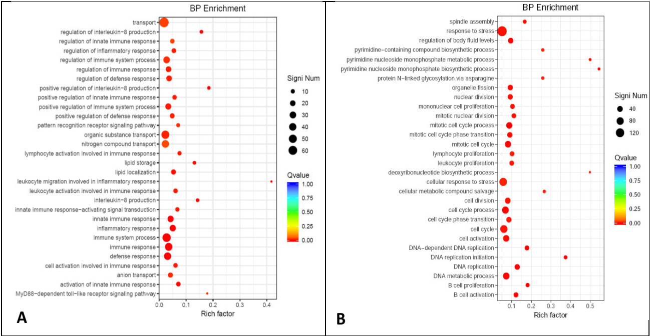
Fig. 2. Enriched functions in BP category of GO annotation for up-regulated (A) and down-regulated (B) DEGs of adult SCTs as compared with cubs. Notes: The Y-axis represents the function annotation information and the X-axis represents the Rich factor corresponding to the function (The number of DEGs annotated to the function divided by the total number of genes annotated to the function). The Qvalue is represented by the dot color (The closer the color to red, the smaller the Qvalue is). The number of DEGs included in each function is represented by the size of the dot.
