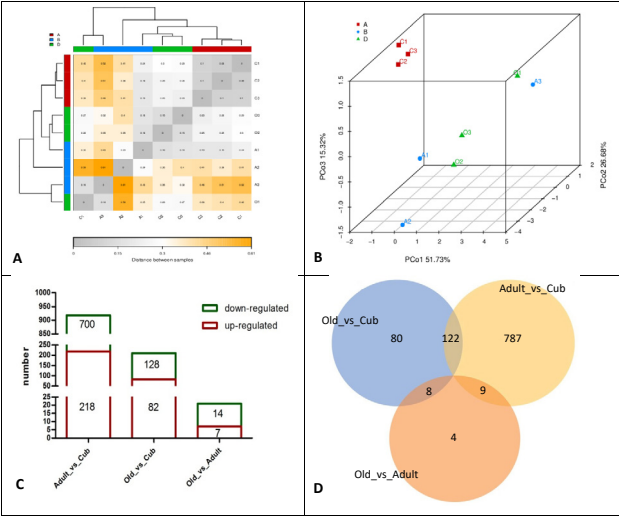
Fig. 1. Profile of the blood transcriptome of SCT. (A) Distance heatmap of all samples based on gene TPM value. (B) PCoA of all samples based on TPM value. (C) Histogram of DEGs in each group (the red box represents up-regulated DEGs, and the green box represents down-regulated DEGs. (D) Venn diagram of the number of DEGs among 3 groups.
