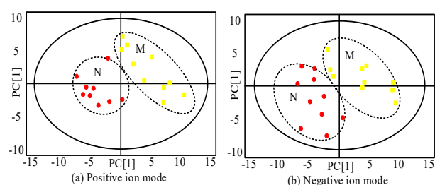
Fig. 3. PCA analysis of HAPC model.
