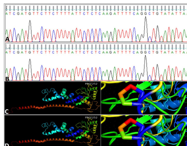
Fig. 2. Mutational analysis of the cadherin gene sequence deduced from PBW and in-silico structure predictions. (A, B) deduced nucleotide sequence of reference cadherin sequence available in GenBank and query sequence depicting no change (C, D) protein structure of reference sequence and deduced sequence of cadherin gene from local PBW isolate showing no change in protein structure.
