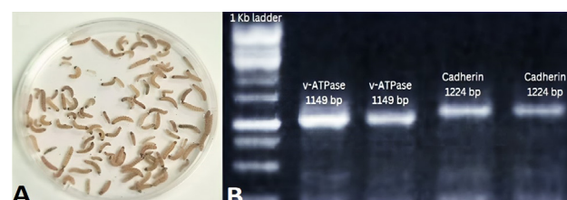
Fig. 1. Amplification of Cadherin and v-ATPase gene fragments from PBW local isolate. (A) The selected pink bollworms for screening (B) The amplified fragments of v-ATPase (~1149 bp) and Cadherin ~1224 bp.
