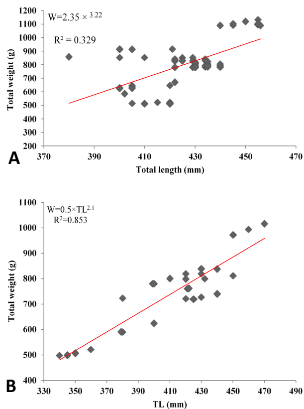
Fig. 4. Length weight relationship of male (A) and female (B) A. maculatus in monsoon.
