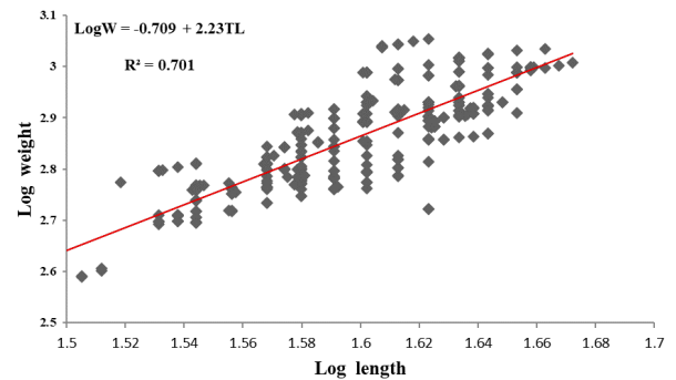
Fig. 1. Length/weight relationship in combined sex of A. maculatus .
