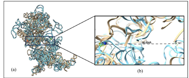
Fig. 5. Zoomed superimposed 3D structures of whole 16S rRNA specifying position 141A>G. (a) Superimposed chains reference yellow and altered blue. (b) Zoomed 141A>G with distance i.e. , 86.004Å.
