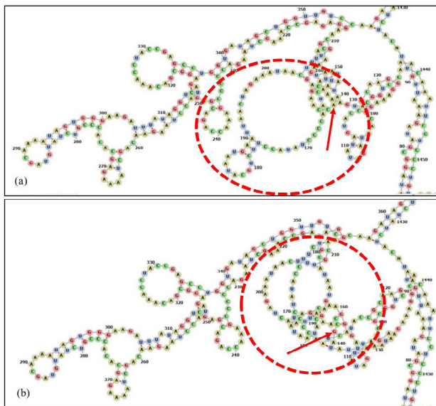
Fig. 4. RNA Fold structure of 16S rRNA molecule and impact of a single 141A>G variation. (a) Reference structure; (b) Altered structure. The red encircled area specifies the structural variation.
