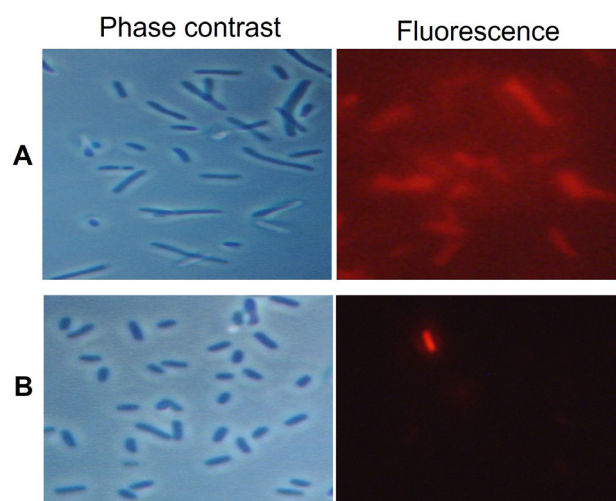
Fig. 3. Representative fluorescence microscopy images E. coli JM83 containing the SOS inducible mCherry based construct treated with MMC for two hours (A), and uninduced cells (B).
