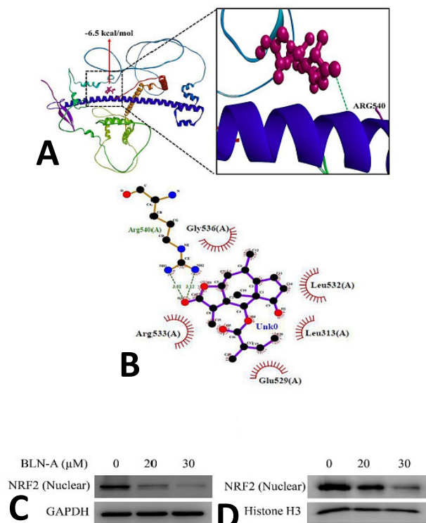
Fig. 3. BLN-A is predicted to bind with NRF2 and inhibits its nuclear translocation. (A) Molecular docking studies showed that BLN-A bind with DNA-binding domain of NRF2 by H-bond. (B) 2D- representation obtained by Ligplot+ revealed hydrogen bonding and other hydrophilic interactions among BLN-A and NRF2. (C) NRF2 expression in nuclear extract of BLN-A treated A549 cells. (D) NRF2 expression in nuclear extracts of BLN-A treated Hey-T30 cells.
