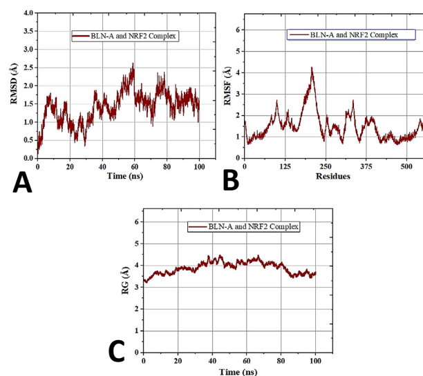
Fig. 4. MD simulation analysis of BLN-A and NRF2 complex: (A) RMSD, (B) RMSF, (C) RG values remained within optimal range depicting stability and compactness of BLN-A and NRF2 complex over 100ns.
