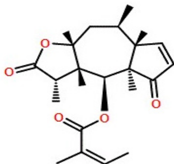
Fig. 1. Chemical structure of Brevilin A.
