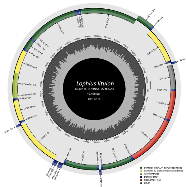
Fig. 1. Organization and characterization of the yellow goosefish mitogenome.
