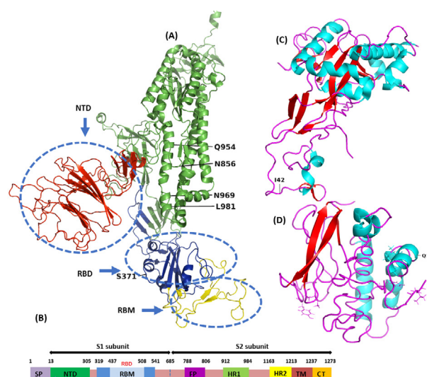
Fig. 2. Locations of unique and most common mutation patterns in spike, NSP14, and membrane proteins of Omicron variants. (A) Spike protein. (B) Domain organization of spike protein. NTD: N-terminal domain, RBD: receptor binding domain, RBM: receptor binding motif, FP: fusion peptide, HR: Heptapeptide repeat sequence, TM: transmembrane region, CT: cytoplasmic tail. (C) NSP14 and mutation in the loop region of Omicron. (D) Membrane protein and location of Q19 mutation.
