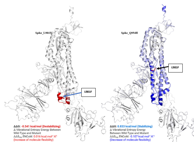
Fig. 4. Mutation effect on spike protein stability and flexibility. Spike_Q954H and Spike_L981F mutations locations and flexibility effect has been shown with arrow. Effect on surrounding residues are red (increase flexibility) and blue (decrease flexibility).
