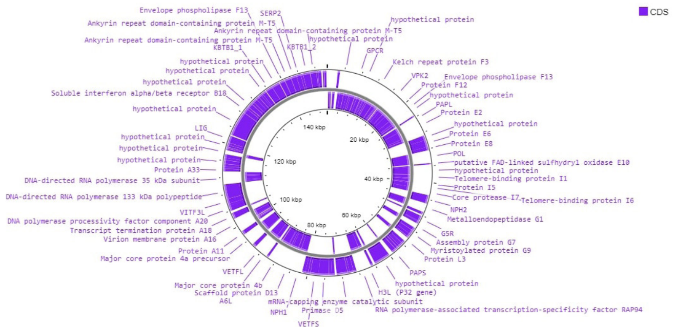
Fig. 1. Annotation of LSD by Prokka and visualized in Proksee. The circular diagram represents the annotated genome of LSDV. The outermost ring indicates coding sequences (CDS) in purple. Key genes and hypothetical proteins are labeled around the periphery of the circle. The innermost rings display various features of the genome, including the positions and density of the CDS.
