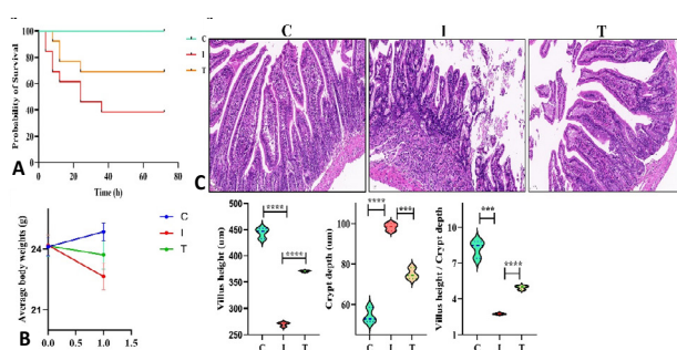
Fig. 3. The in vivo inhibitory effect of SUP on E. coli . (A) Survivorship curve, (B) average body weights, (C) intestine pathologic analysis. Scale bar 50 \mu m. Significance is presented as *** P < 0.001 and **** P < 0.0001 ; data are presented as the mean \pm SEM.
