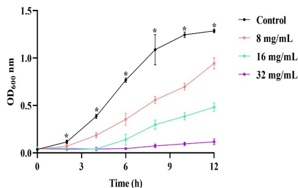
Fig. 1. The inhibition effect of SUP on the growth curve of E. coli . Data are described as the mean \pm SEM ( n = 3 ).
