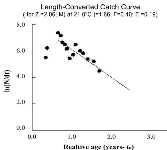
Fig. 5. Length converted catch curve for L. rohita from the Indus River.
