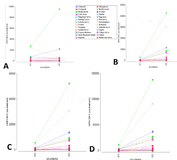
Fig. 4. Abundance of species (individuals/m 3 ) in (A) autumn inter monsoon (October and November), (B) north east monsoon (December, January and February), (C) spring inter monsoon (March and April), (D) south west monsoon (May to September) in Sandspit.
