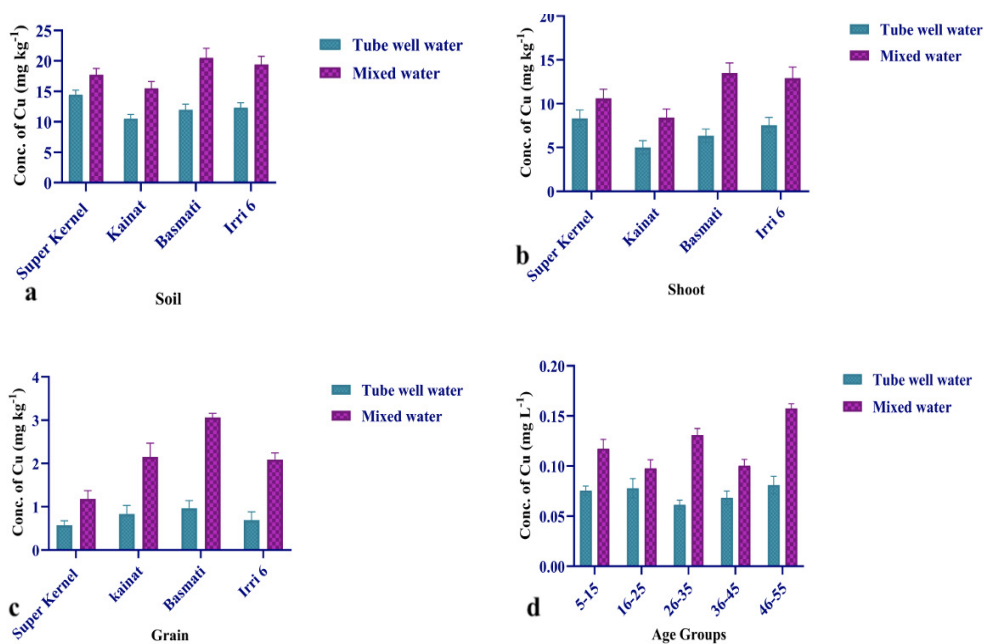
Fig. 3. Cu concentration in soil (a); rice shoot (b); rice grain (c) and human serum samples (d).
