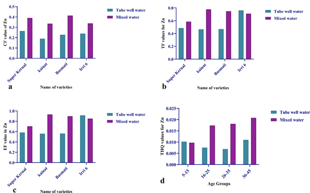
Fig. 4. Contamination factor (a); transfer factor (b); enrichment factor (c); target hazard quotient (d) of Zn in four varieties of rice irrigated with tube well water and mixed water.
