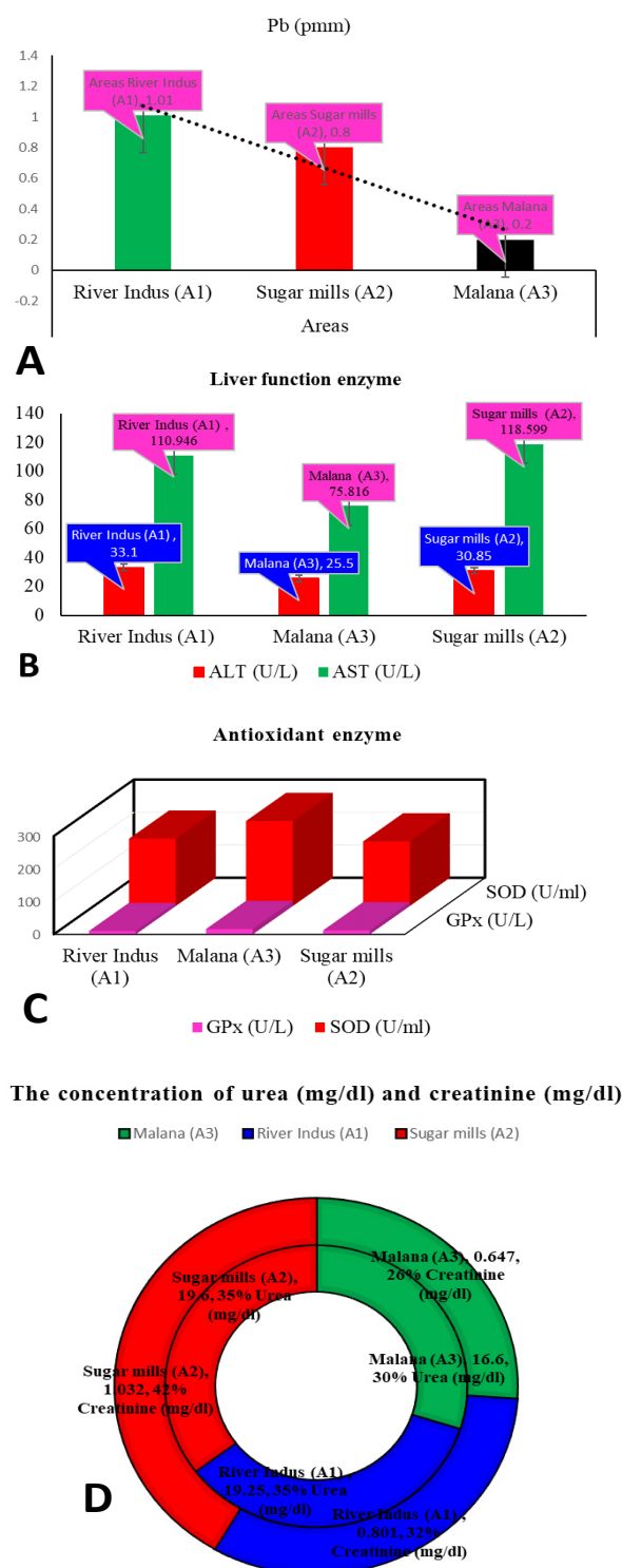
Fig. 1. The level of Pb (A), liver function enzyme (B); antioxidant enzyme (C), and renal function parameters (D) in blood serum of Damani sheep grazing in the three area (A1, A2 and A3).
